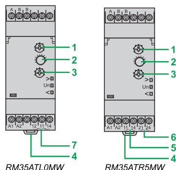
RM35ATL0MW
