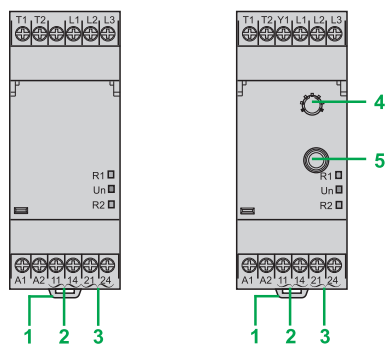
RM35TM50MW
