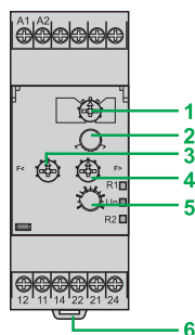
RM35HZ21FM
