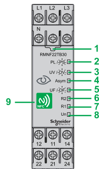
NFC Control Relay
