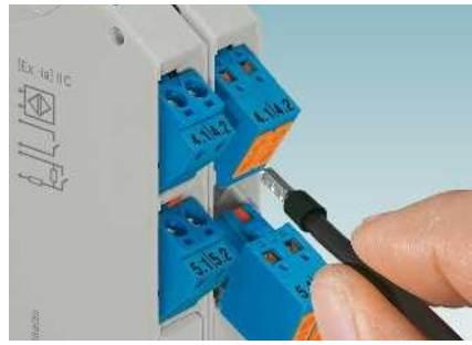
Connection terminal blocks with integrated test sockets and polarity reversal protection
