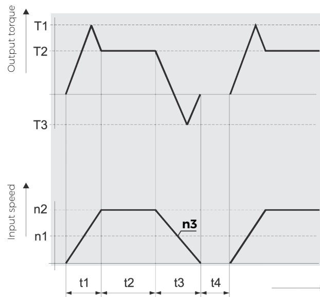
Fig. 4.1: Duty cycle
