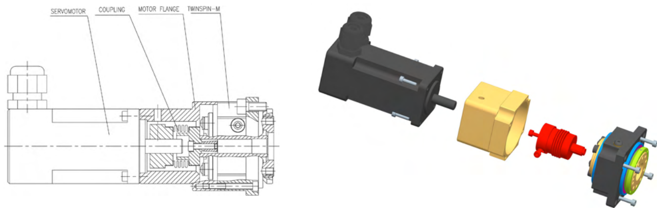
Fig. 5.4.1b: Shaft connection with flexible coupling
