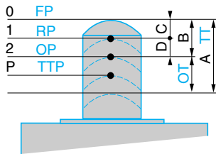
Linear movement (plunger)
