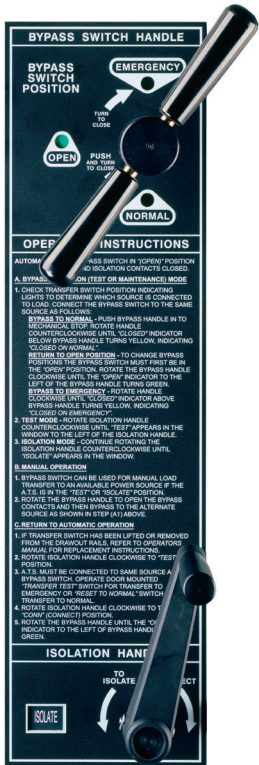
Bypass and isolation controls and operating instructions
