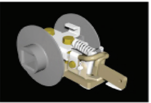
Finite element analysis and 3-D computer models (left) create components that are specifically designed for transfer switch duty. Durability and reliability are built in. See page 27 for more information on ASCO design innovations.
