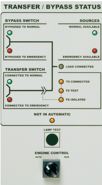
ASCO Transfer/Bypass Status Panel
