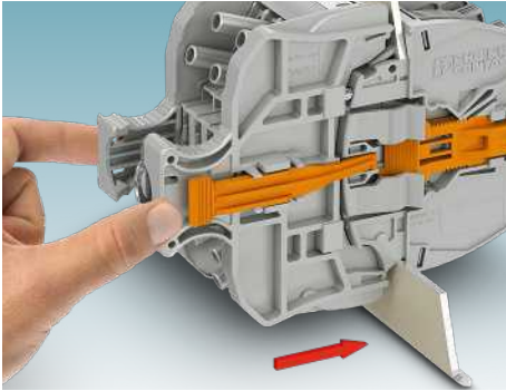
By plugging in and latching the test plug, all test contacts are securely contacted in accordance with the test setup.
