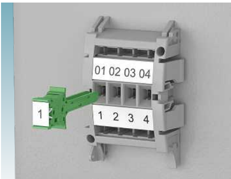
Service connectors are available with varying numbers of positions for special switching operations.
