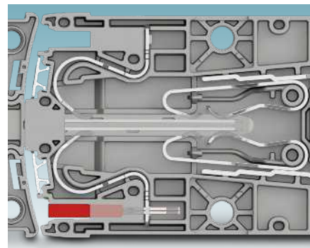
S-plate – late switching point
