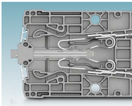
M-plate – delayed switching point
