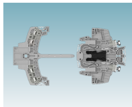
FAME 3 auxiliary contact for status recognition
