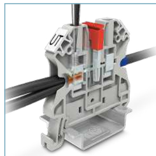
Terminal block with UT screw connection
