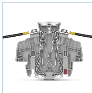
FAME 3 plug-in test socket with RSC ring cable lug connection
