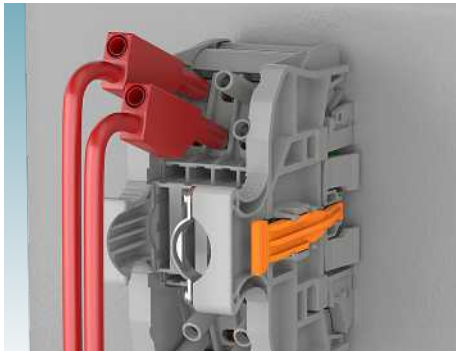
Space-saving test points with offset test sockets. Multi-position test cables can be securely fixed via a strain relief system.
