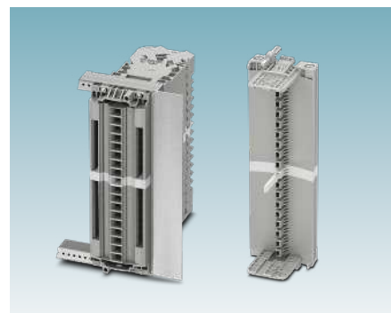
Plug-in test socket and blind plug with status contact
