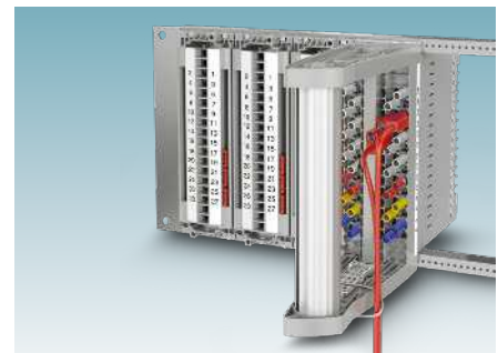
Test plug of the FAME 3 RACK system
