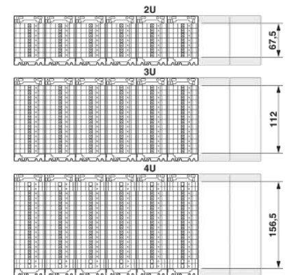
Rack units of the FAME 3 RACK
