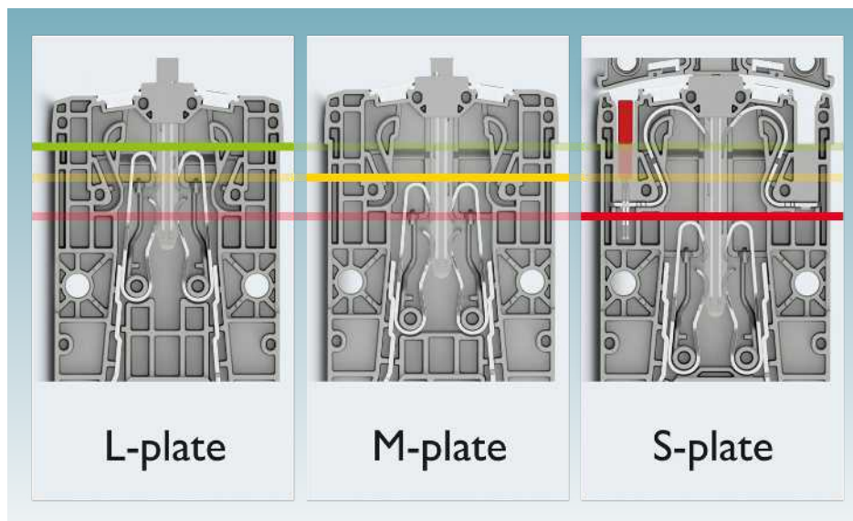
Switching points of the FAME 3 RACK plug-in test system
