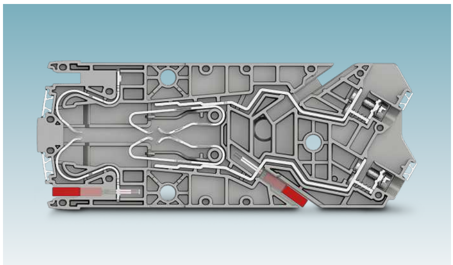
Single plate of the FAME 3 RACK plug-in test socket
