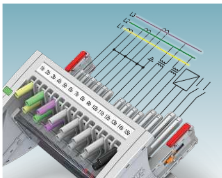
FAME 2 test plug
