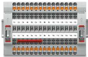
Plug-in test socket, blind plug
