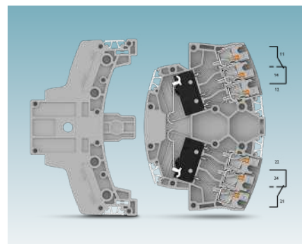
Plug-in test socket with status indicator
