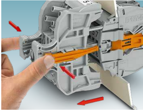
The latching is released by actuating the orange latching rockers. Unplugging the test plug will restore the original signal connections.
