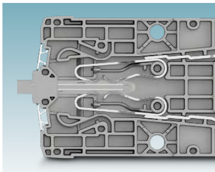
L-plate – early switching point
