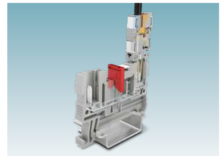
Terminal blocks with plug-in connection
