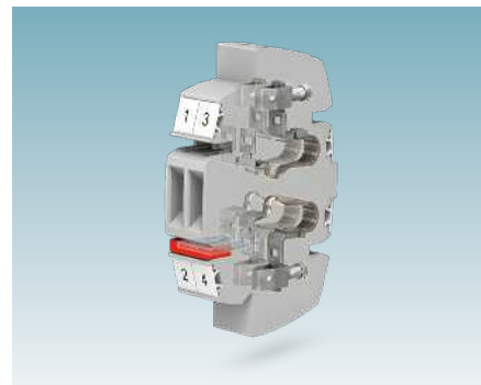
FAME 1 transformer short circuit
