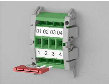
The automatic, leading transformer short circuit is configured with standard plug-in bridges in the plug-in test socket. The positioning of the short-circuit bridges on the outside of the control cabinet is clearly visible.
