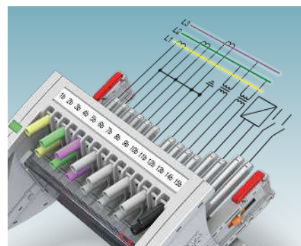
Status indicator
