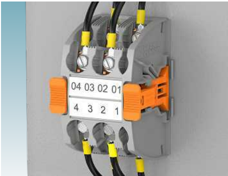
The plug-in test sockets have screw connection technology for ring cable lugs.
