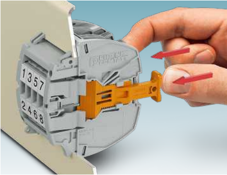
The plug-in test socket positioned in the cutout is fixed in place without screws by pressing on the two orange actuating elements.
