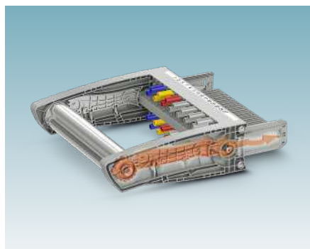
FAME 3 RACK rotary handle mechanism
