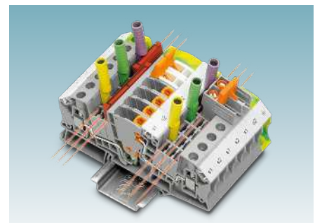
Transformer terminal block with 6 function shafts
