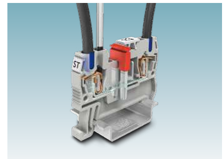
Terminal blocks with ST spring-cage connection
