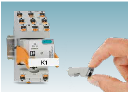
The universal industrial relay system with multifunctional timer module.
