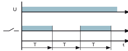
Pulse generator
