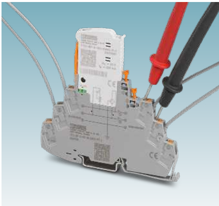
Testing directly at the protective device
