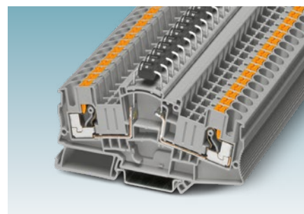
PTME 6-DIO/L-R HV component terminal block
