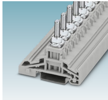
HV M5/1 high-current connector
