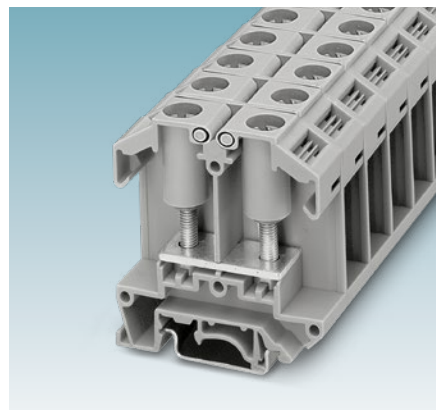
OTTA 6 bolt connection terminal block
