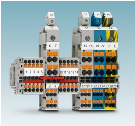
PT 35/4X6/6X2,5 potential collective terminals
