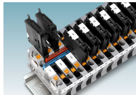
Fuse terminal blocks with fuse holders that can be swiveled
