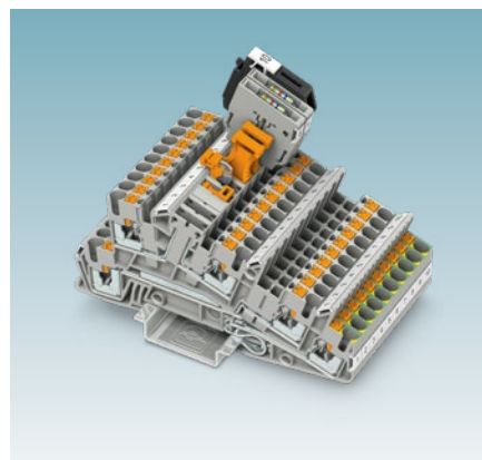
Disconnect and knife-disconnect terminal blocks
