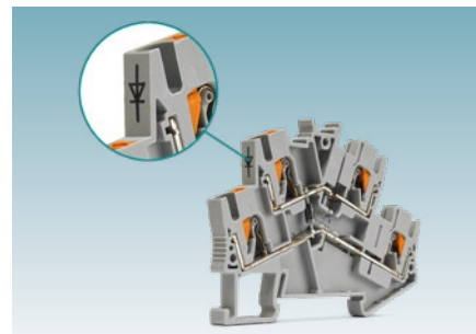
PTTBS 2,5-DIO/O-U component terminal block
