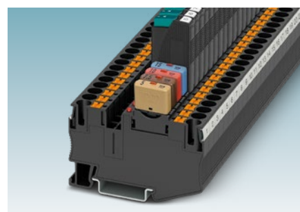
Thermal circuit breakers for overload and short-circuit protection
