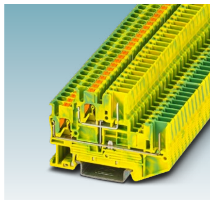
ST 2,5/2P-PE ground terminals
