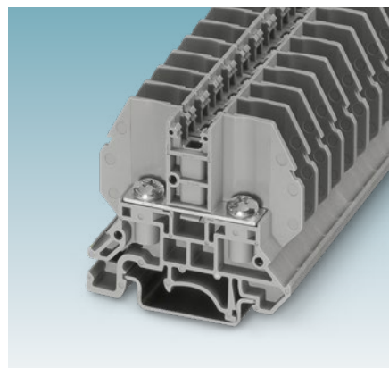
RSC 4 bolt connection terminal block
