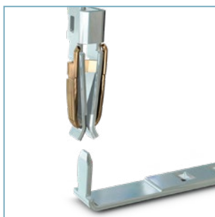
Clamping part of a plug-in terminal block
