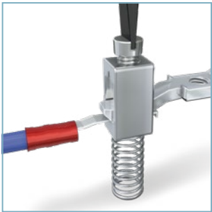
Connection chamber of USST terminal blocks
