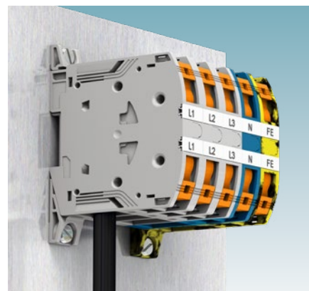
PTPOWER 95 as a block version
