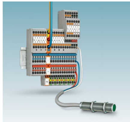
PTIO sensor/actuator terminal blocks
