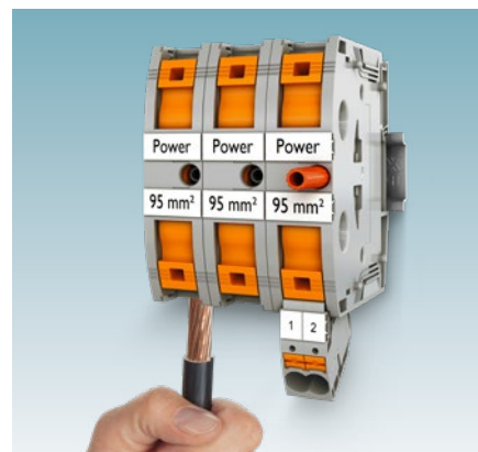
PTPOWER 95 with test point in the middle
