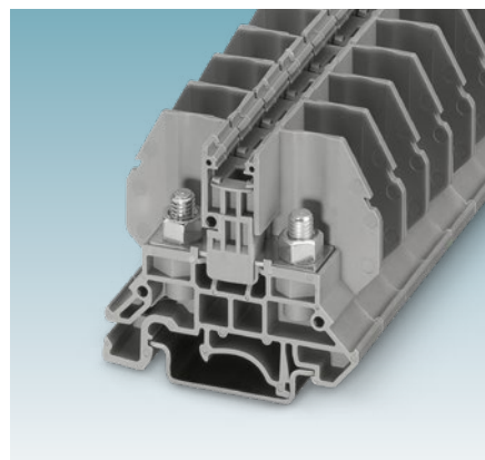
RBO 10 bolt connection terminal block
