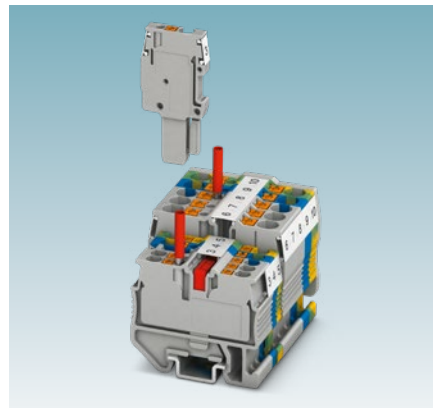
MPT 2,5 miniature terminal blocks
