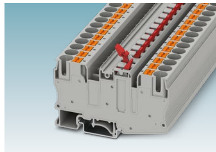
PT 10-MTL lever-type knife-disconnect terminal blocks
