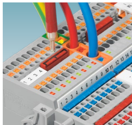
PTIO feed-in terminals
