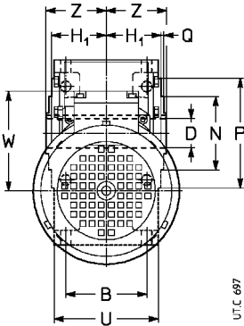
MR 2IV 40 ... 81
