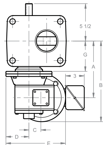
REDUCER DIMENSIONS
