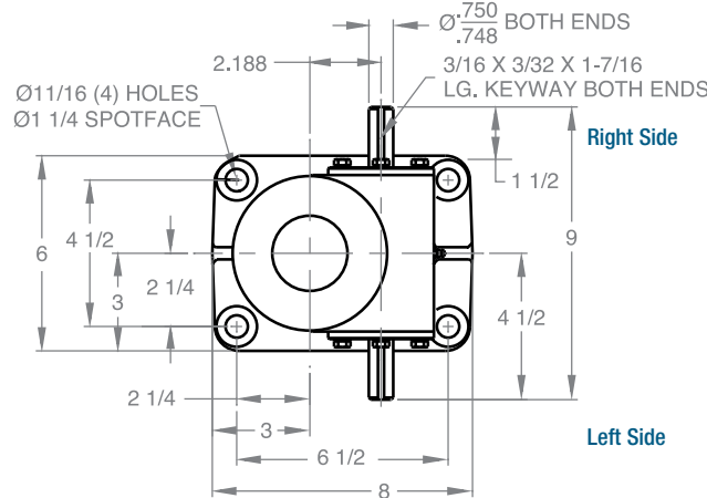
TYPE 2 LOAD PAD
