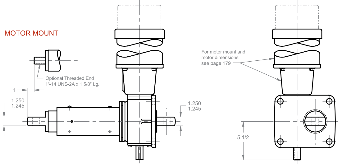
REDUCER DIMENSIONS
