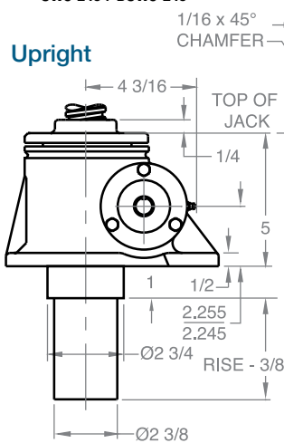
TYPE 1 PLAIN END
