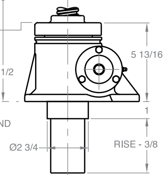
TYPE 4 MALE CLEVIS END
