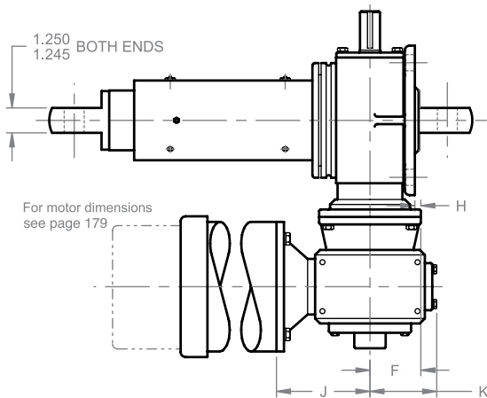
REDUCER DIMENSIONS
