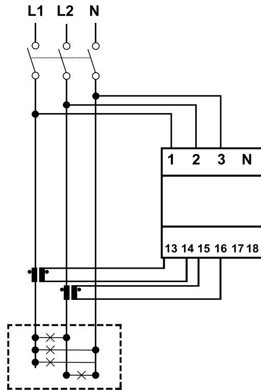
Bi-phase system
