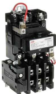
Open starters
